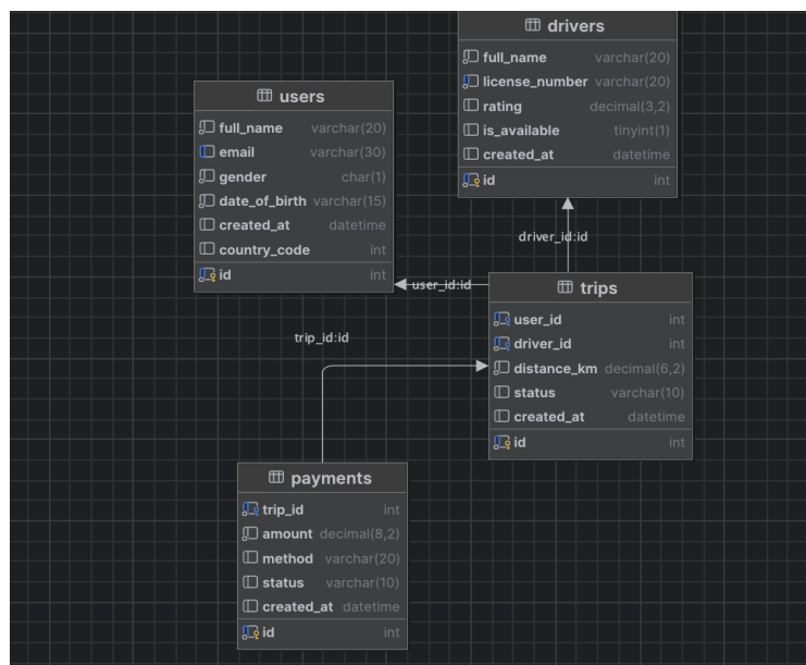
Figure 1 — Entity Relationship Diagram for the Uber Database
